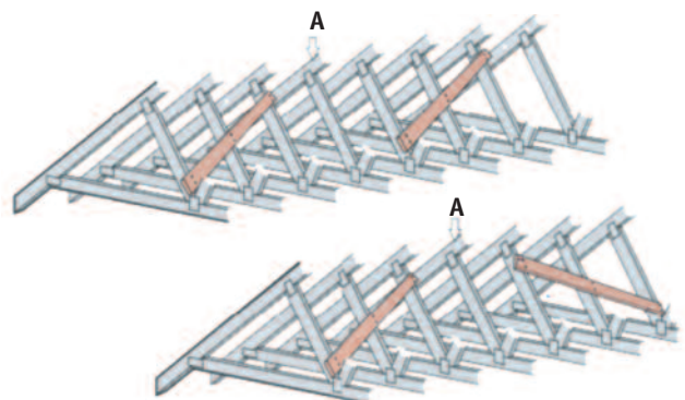
Fig. 8 Alternative fixing arrangement for chevron braces (truss span over 8m)
