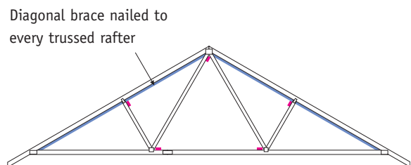
Fig. 4 Position of diagonal wind braces
