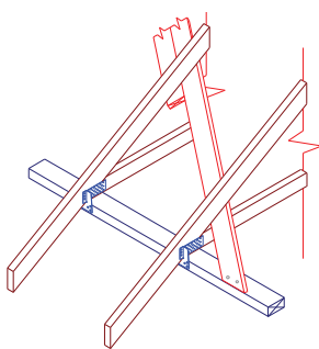
Rafter brace nailed to wall plate.
