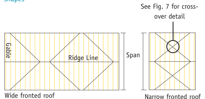
Fig. 5 Plan of rafter diagonal bracing on differing plan shapes
