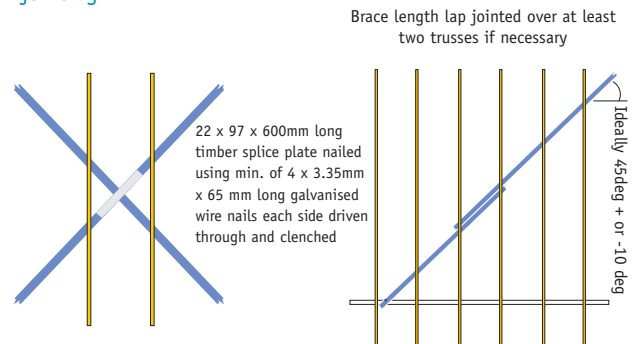
Fig. 8 Alternative fixing arrangement for chevron braces (truss span over 8m)
