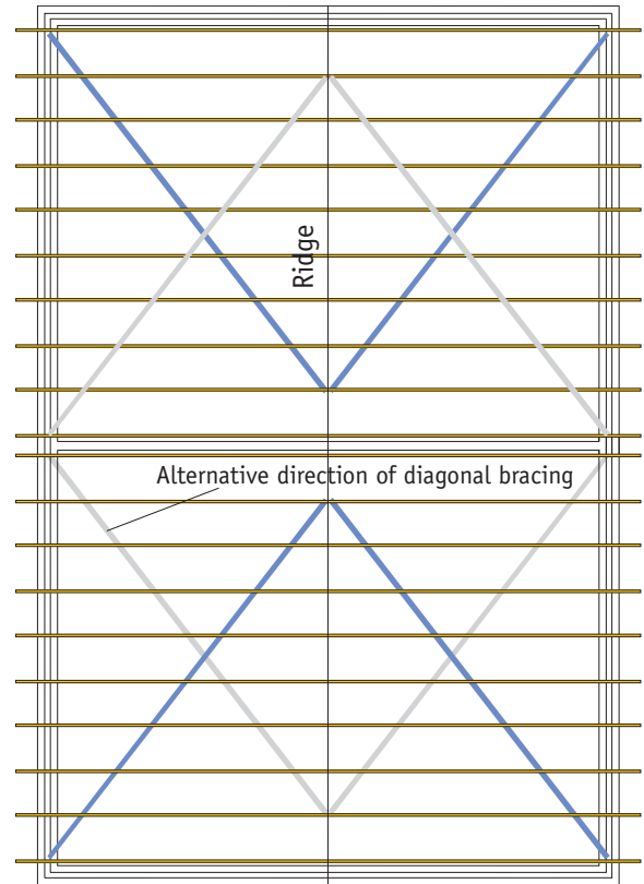
Fig. 7 Splicing of intersecting diagonal braces and end jointing
