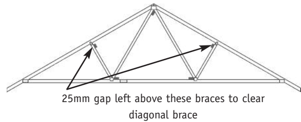
Fig. 2 Positions of longitudinal braces
