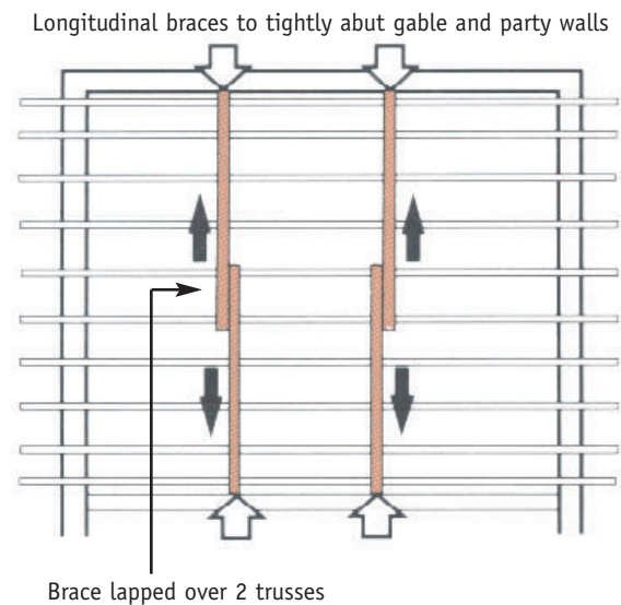
Fig. 3 The fixing of longitudinal braces
