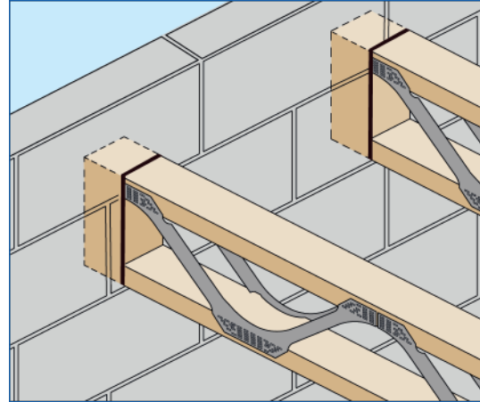
Block work to continue between Posi-Joists to provide restraint. Note: This is not allowed on solid external walls
