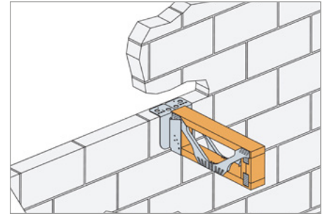
Timber to masonry
